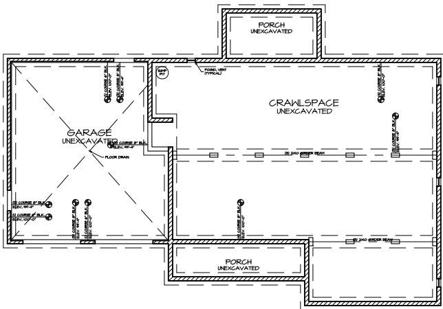
1 FOUNDATION PLAN A-3 SCALE: 1/4"=1'-0"
