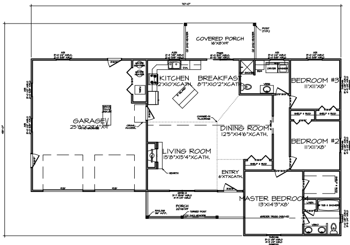
1 FIRST FLOOR PLAN A-4 SCALE: 1/4"=1'-0"
